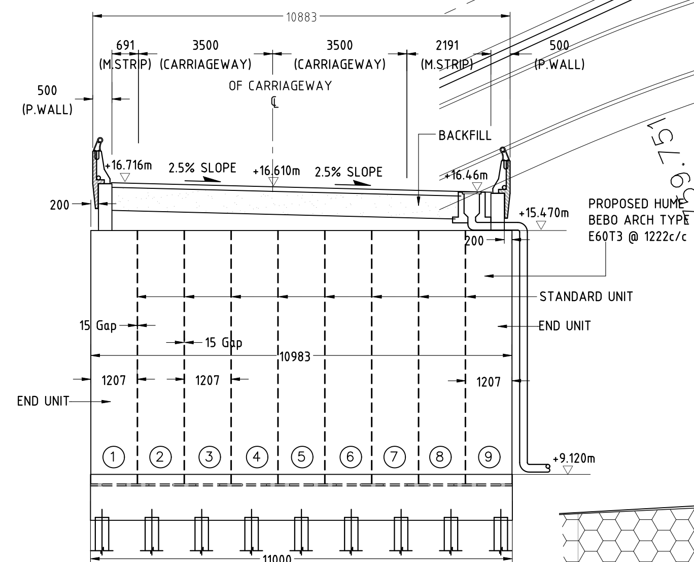
ABUTMENT FRONT ELEVATION - VIEW 'A'
